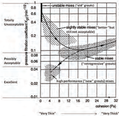
Figure 2. Historical path of development from unstable mixes to contemporary balanced multi-component mixes (modified after De Paoli et al., 1992).
